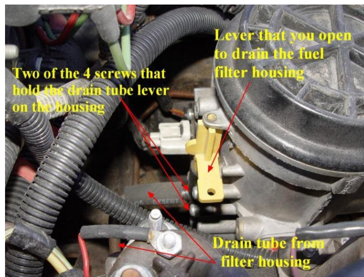
Fuel Drain Assembly view from Passenger side Questions: Send email to Support@dfuser.com Visit us on the web: http://www.dfuser.com
